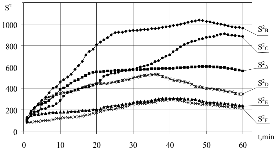
Fig. 2. Dispersion of the temperature of the heated surface of the bearing wall in the computational experiment. S^2_{A-F} - The dispersion of the temperature of the heated surface of the bearing wall in the computational experiment in the configuration of the fire furnace, which corresponds to this index ("A-F" configurations).
