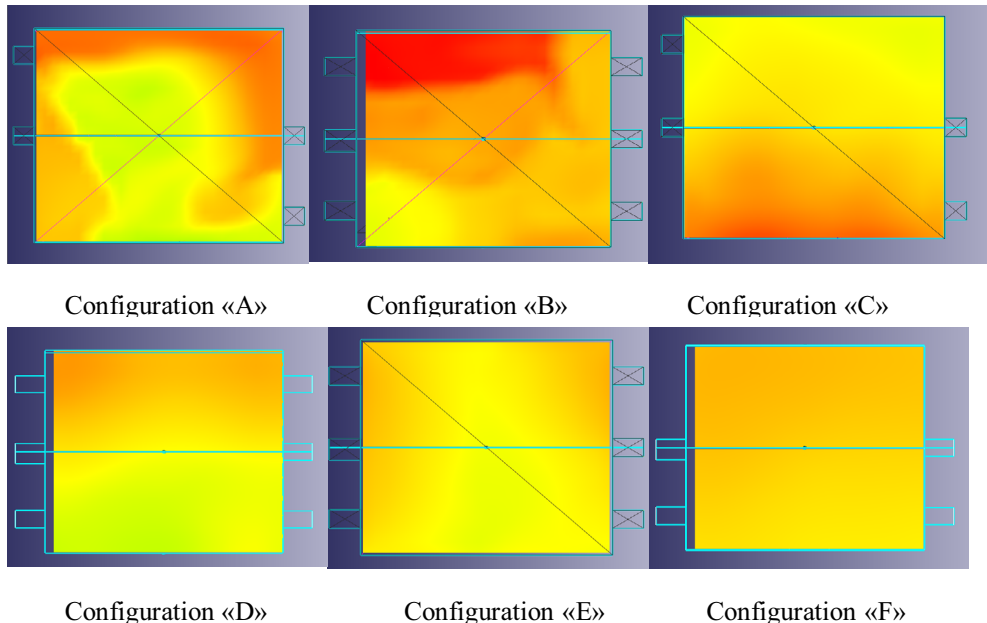
Fig. 1. Temperature gradient at the heated surface of the simulated structures configurations from A to F.
