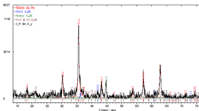
Figure 1 X-ray diffraction pattern of nanopowder containing polyvalent iron oxides obtained by electrical discharge dispersion (EDD).
