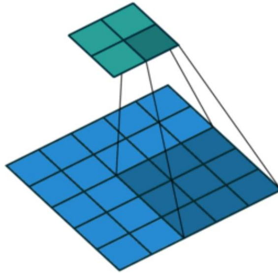
Figure 1. Convolution with a step of 2
