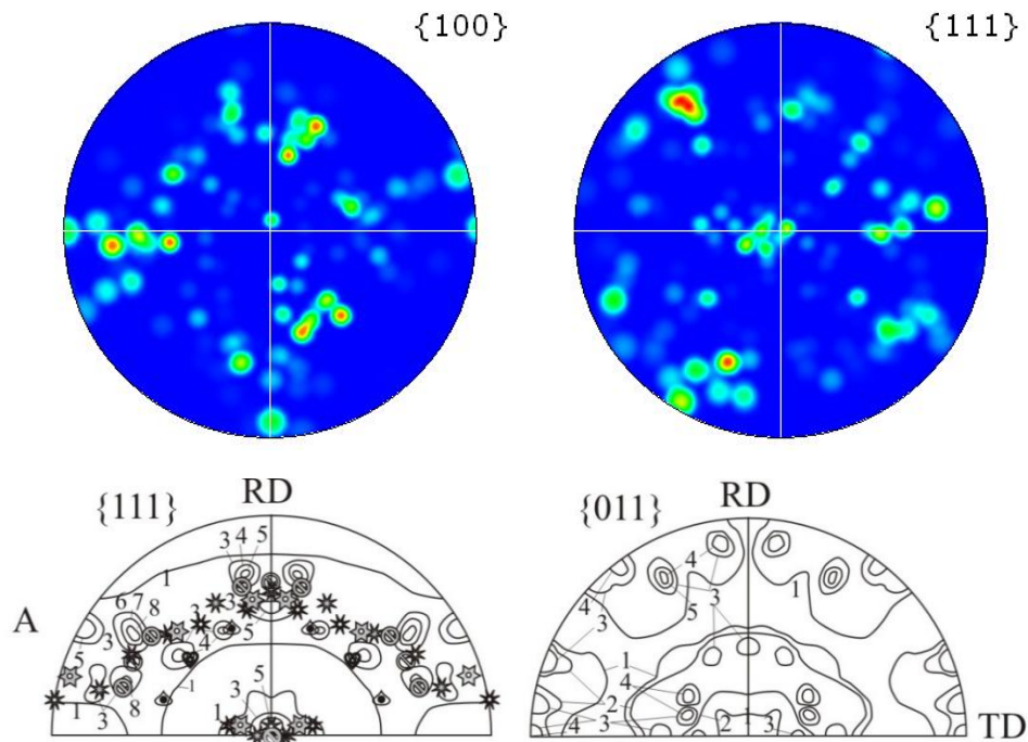
Fig.2. Experimental {001}, {111} and averaged {111}, {011} PFs of the original DC04 steel sheets
