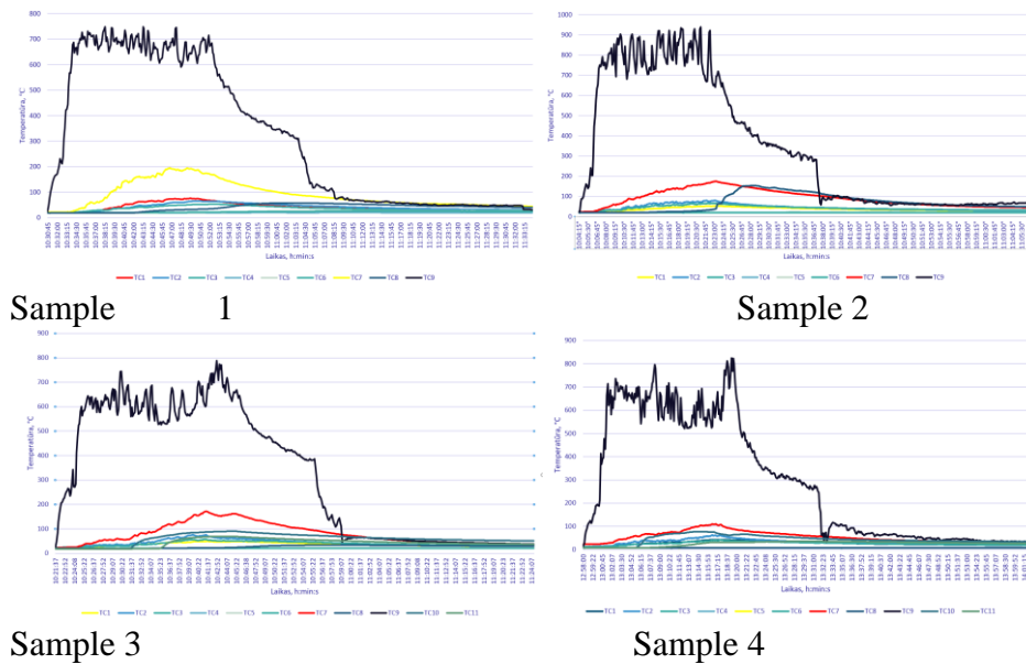
Fig. 5 Samples temperatures
