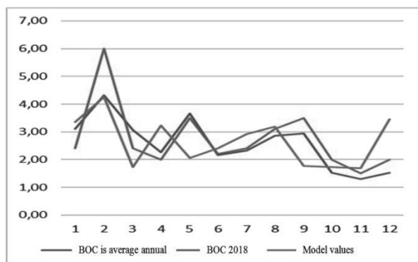
Fig. 4. Dynamics of simulated, average and actual (2018) BOD 5 values (mg/dm 3 )
