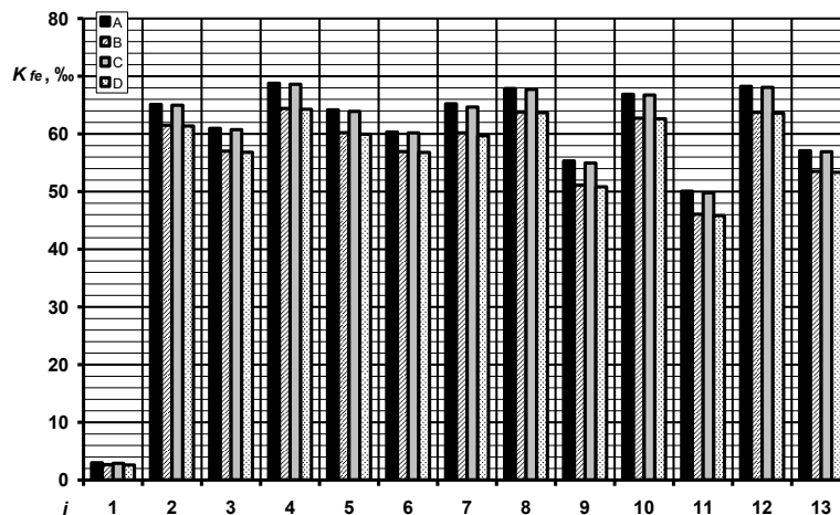
Figure 1 – Distribution of magnitudes of criterion K_{fe} on regimes of standardized steady testing cycle ESC for autotractor diesel engine 2Ch10.5/12
