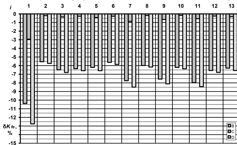
Figure 2 – Distribution of magnitudes of value \delta K_{fe} on regimes of standardized steady testing cycle ESC for autotractor diesel engine 2Ch10.5/12
